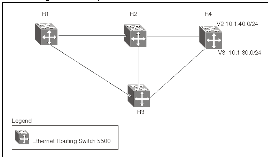
Figure 43 ECMP configuration example
