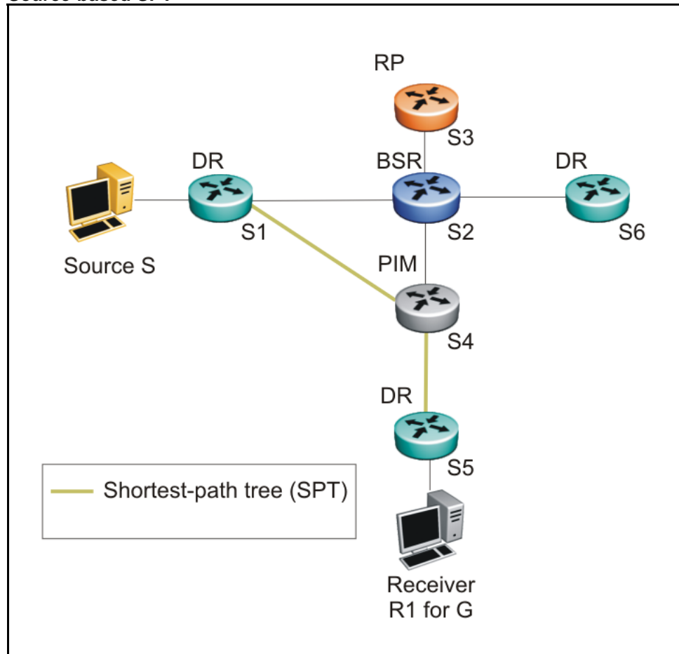
Figure 30 Source-based SPT
