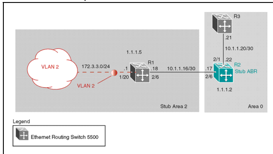
Figure 36 OSPF stub area example
