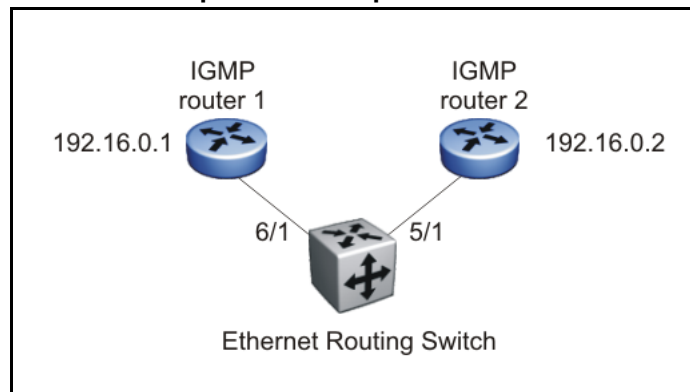
Figure 28 Static mrouter port and nonquerier
