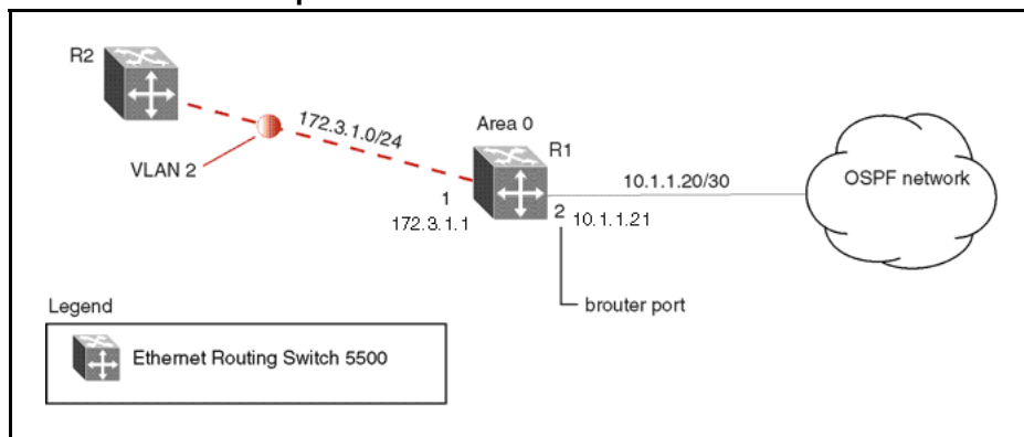
Figure 33 OSPF network example
