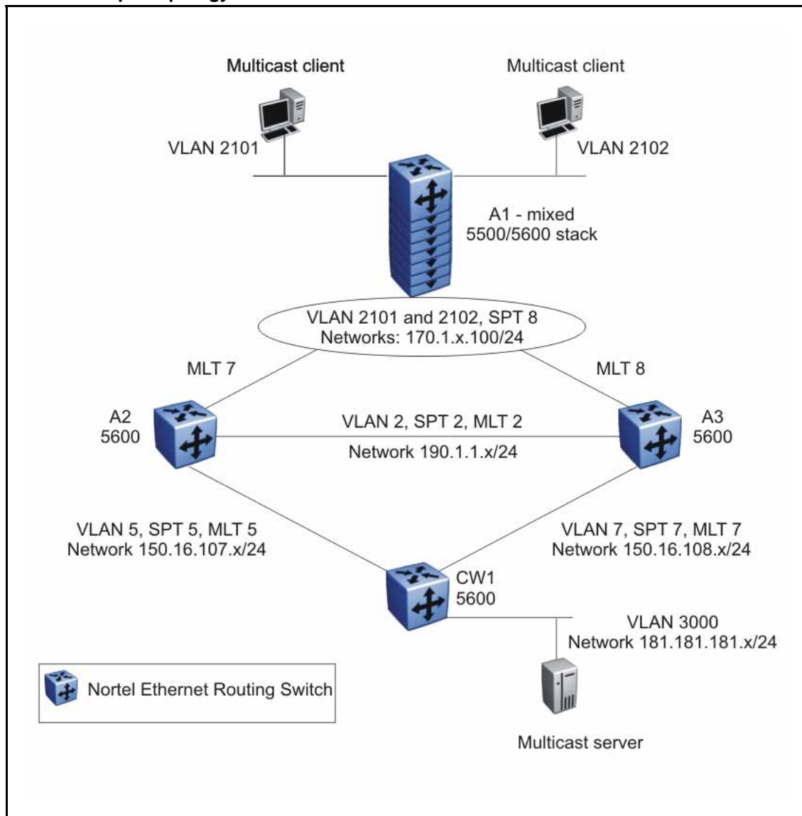
Figure 47 PIM-SM sample topology
