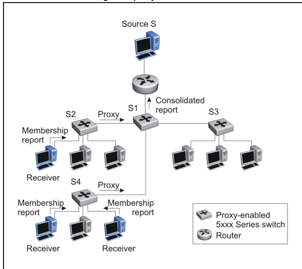
Figure 27 5000 Series switch running IGMP proxy
