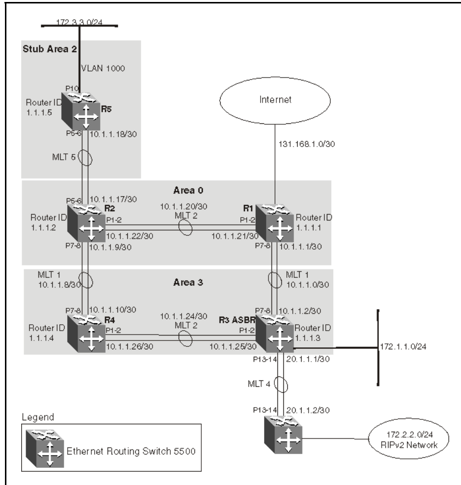
Figure 39 Multi-area complex example
