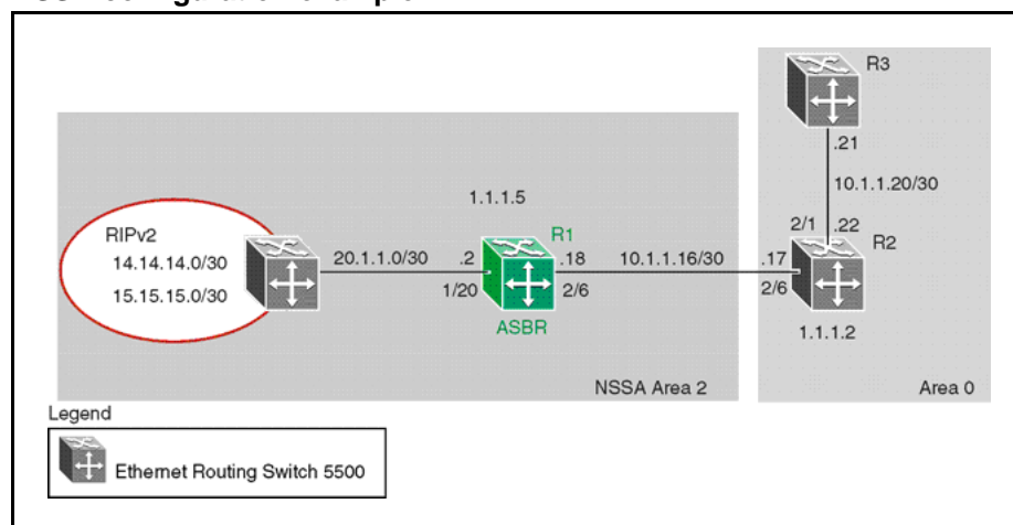
Figure 37 NSSA configuration example
