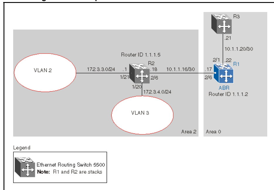
Figure 34 ABR configuration example
