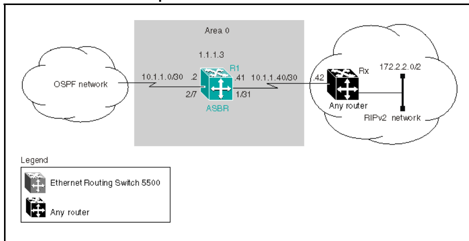
Figure 35 ASBR distribution example
