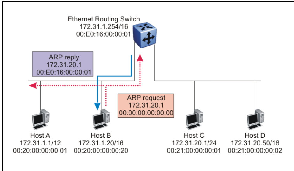
Figure 15 Proxy ARP Operation
