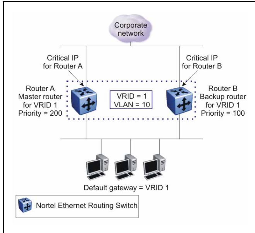
Figure 16 VRRP topology example
