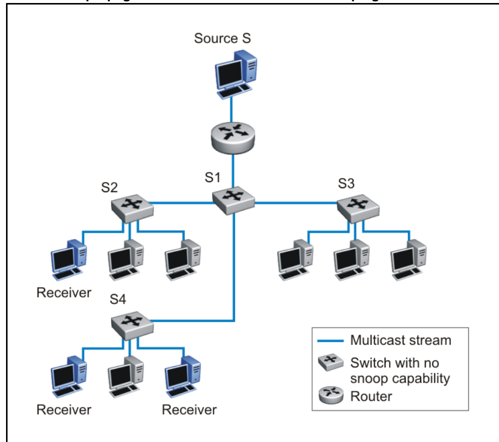
Figure 25 IP multicast propagation on a LAN without IGMP snooping
