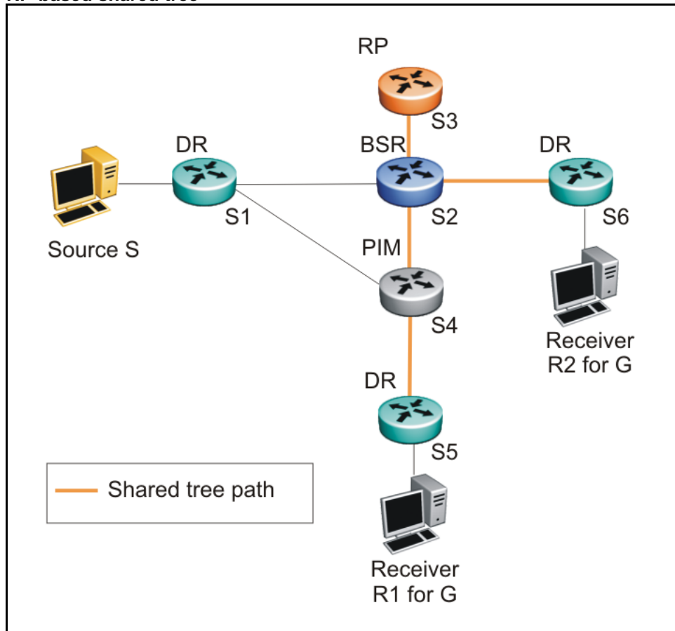
Figure 29 RP-based shared tree
