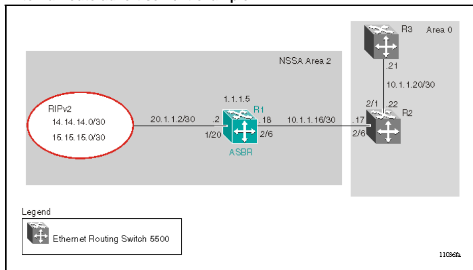
Figure 38 External route advertisement example
