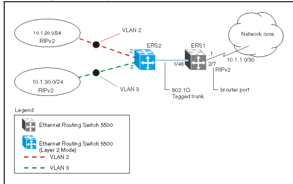
Figure 41 RIPv2 configuration example
