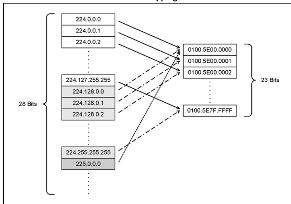
Figure 21 Multicast IP address to MAC address mapping
