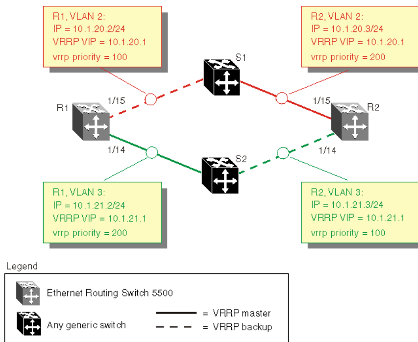
Figure 44 VRRP example topology
