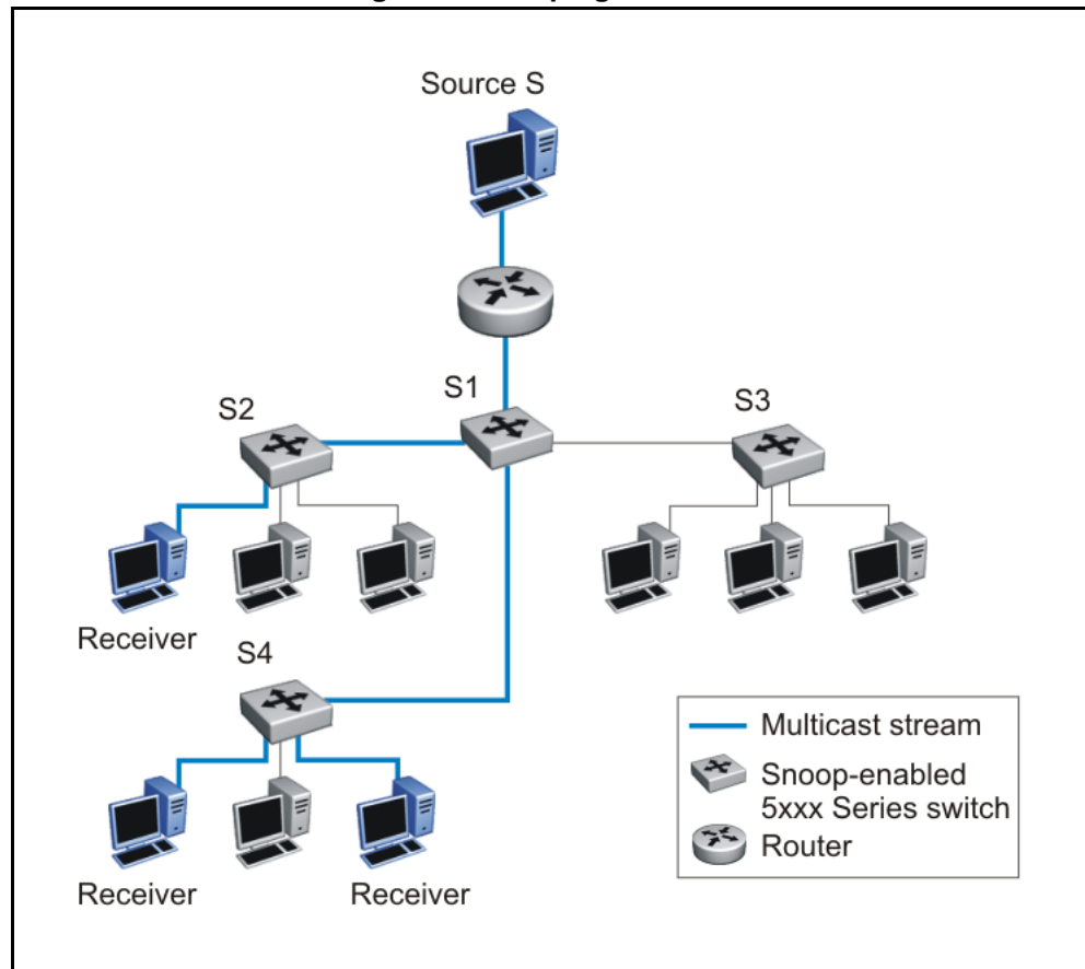
Figure 26 5000 Series switch running IGMP snooping
