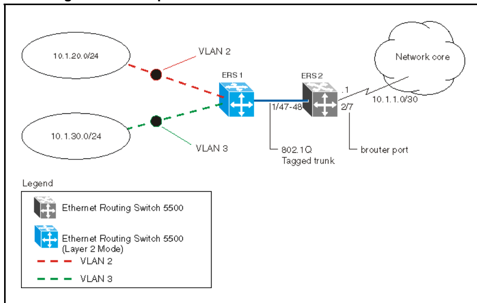
Figure 40 RIP configuration example
