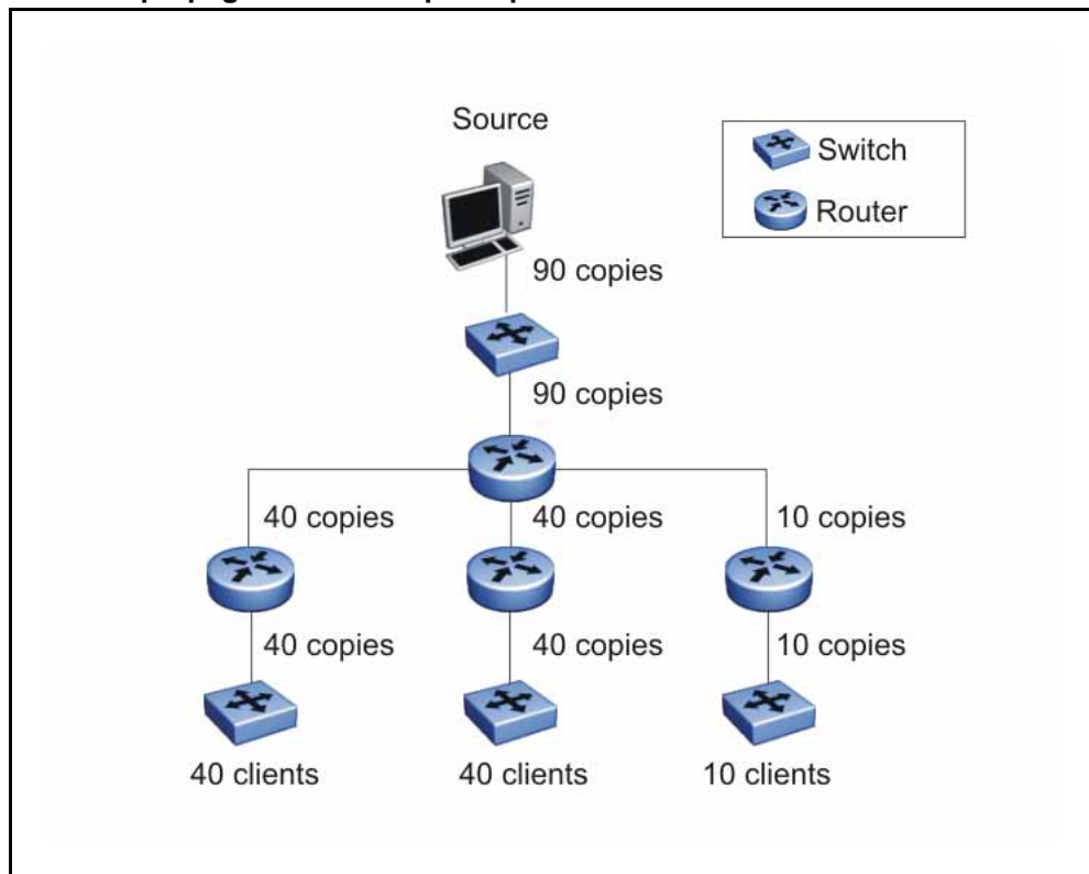
Figure 18 Wasteful propagation of multiple copies of the same unicast stream
