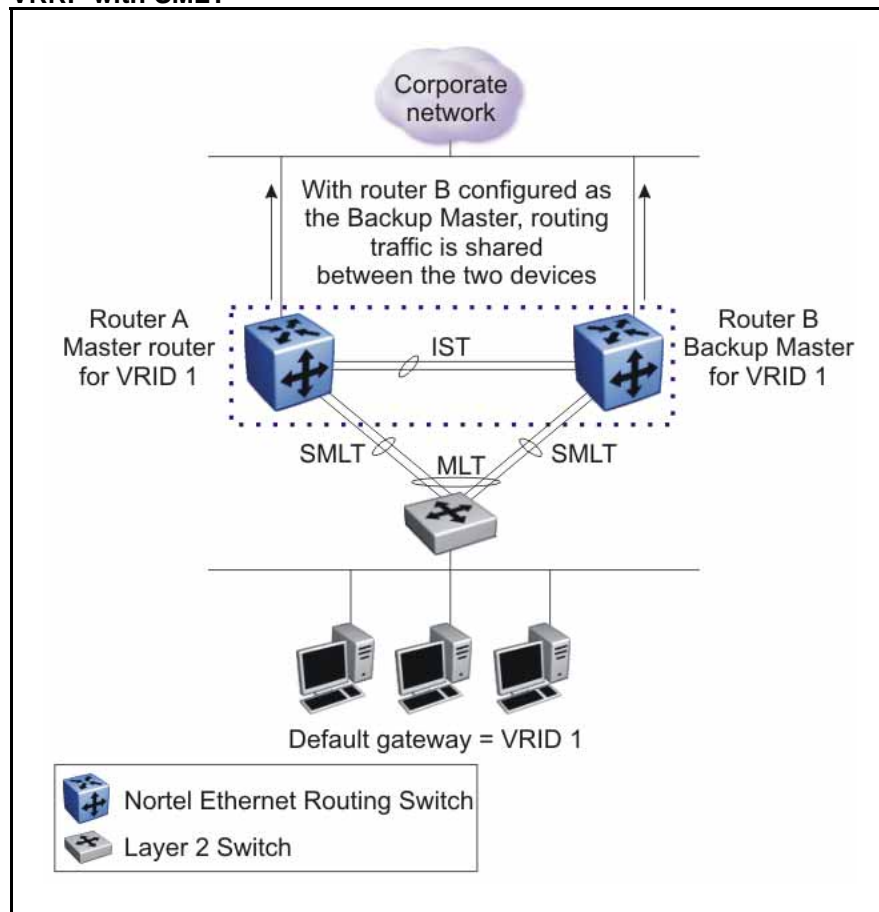
Figure 17 VRRP with SMLT
