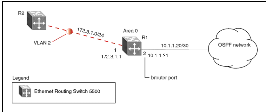
Figure 31 OSPF interface example topology
