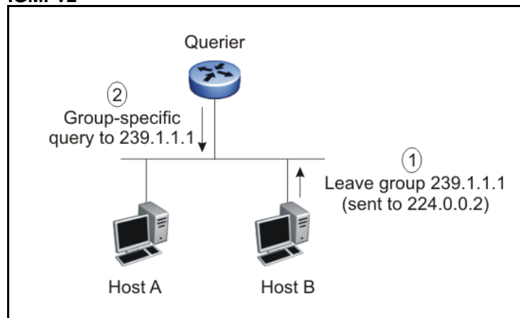
Figure 23 IGMPv2
