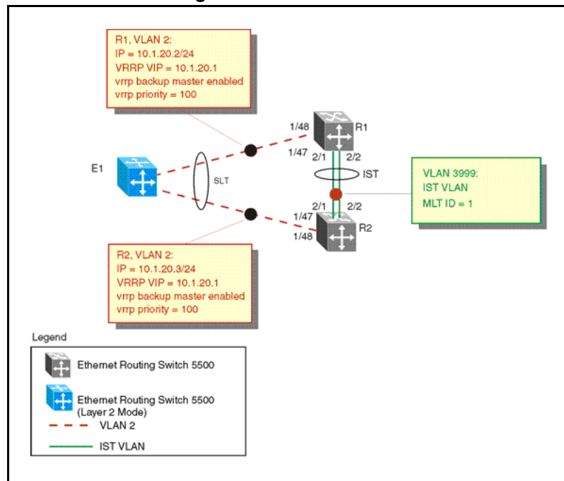
Figure 46 VRRP with SLT configuration
