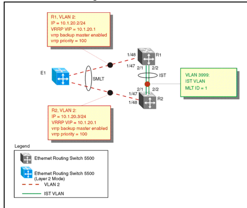
Figure 45 VRRP with SMLT configuration
