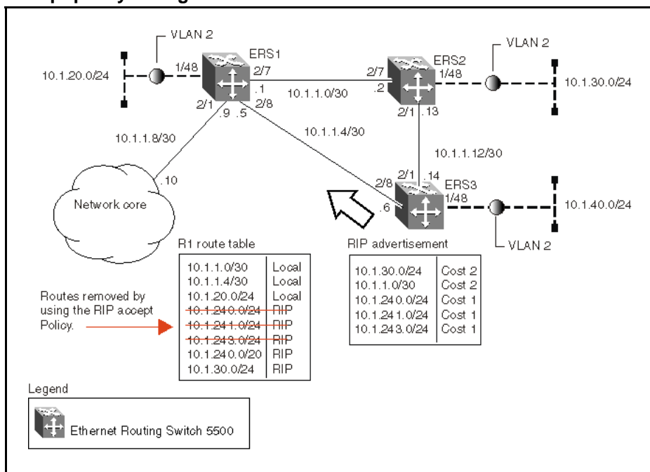
Figure 42 Accept policy configuration
